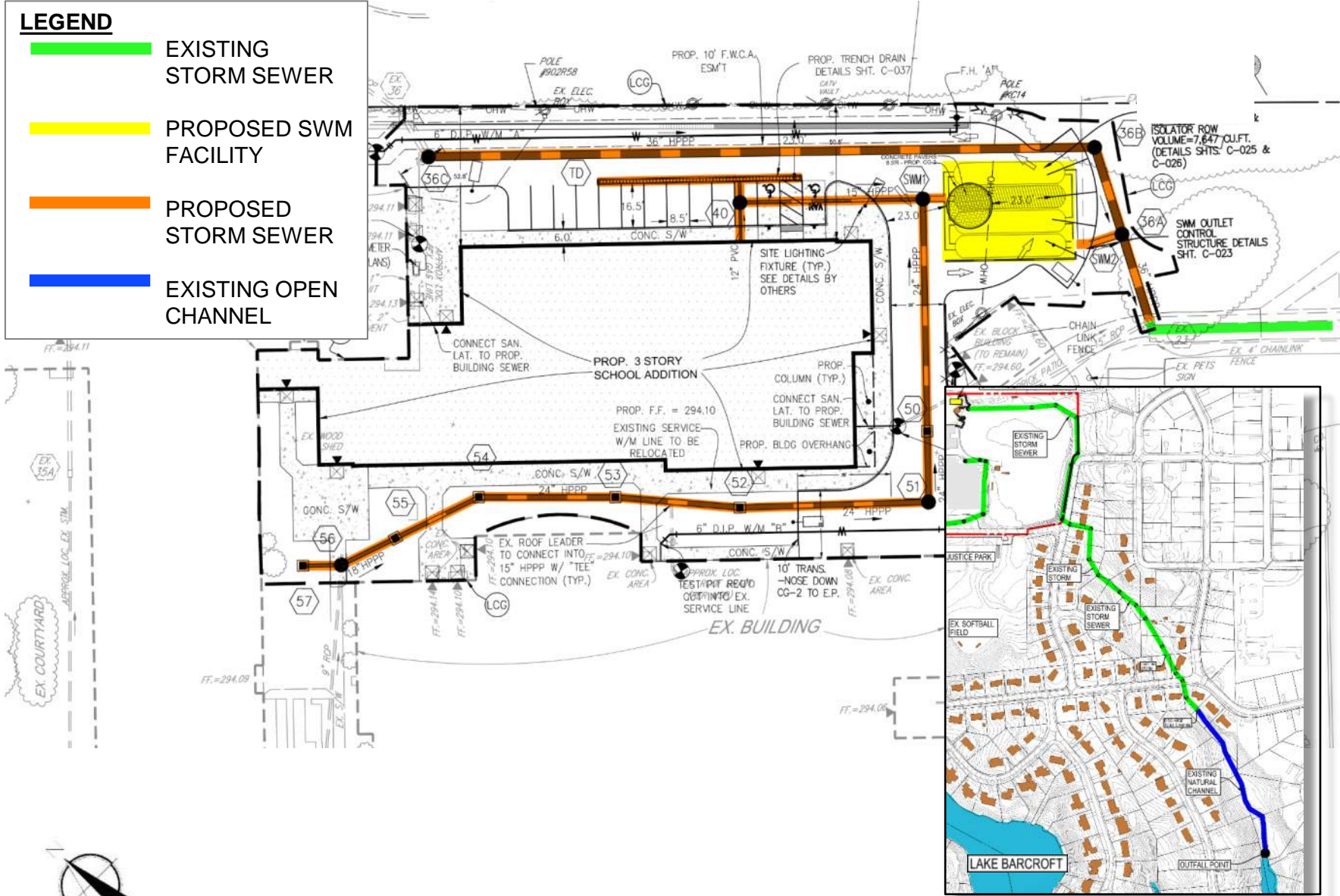
SWM Outfall
