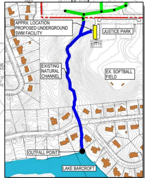
SWM Outfall
