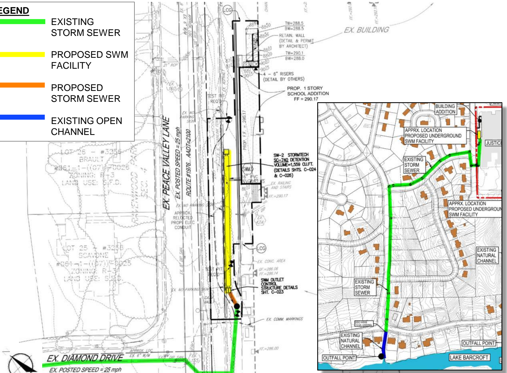
SWM Outfall
